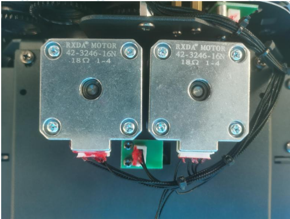
Photo 7: Motor view
