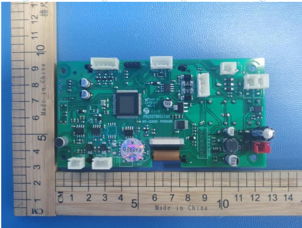
Photo 16: PCB view
