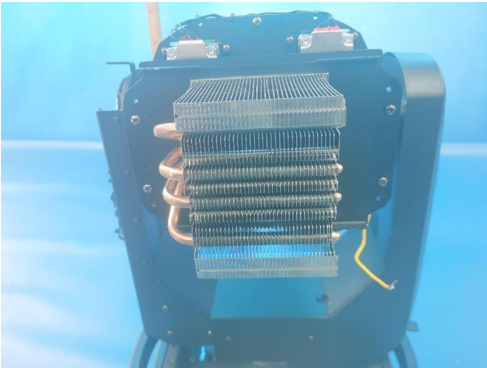
Photo 6: Air-cooling fin view
