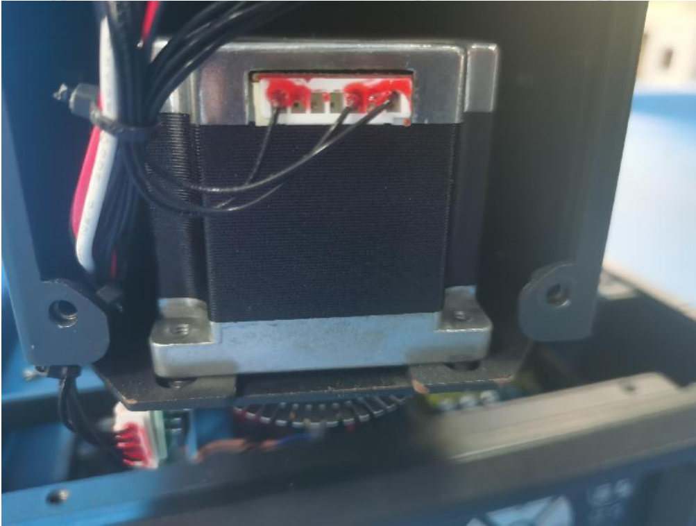
Photo 9: Motor view
