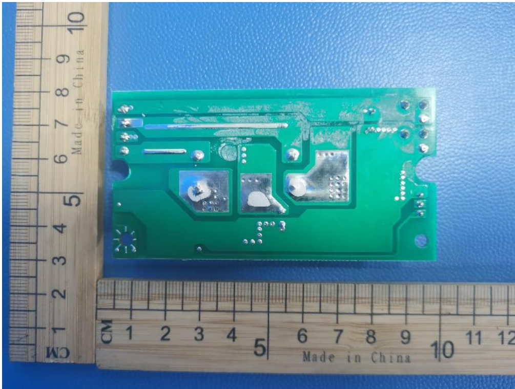
Photo 15: PCB view
