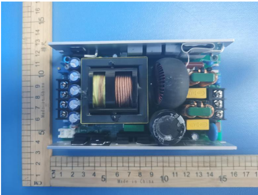
Photo 18: PCB view
